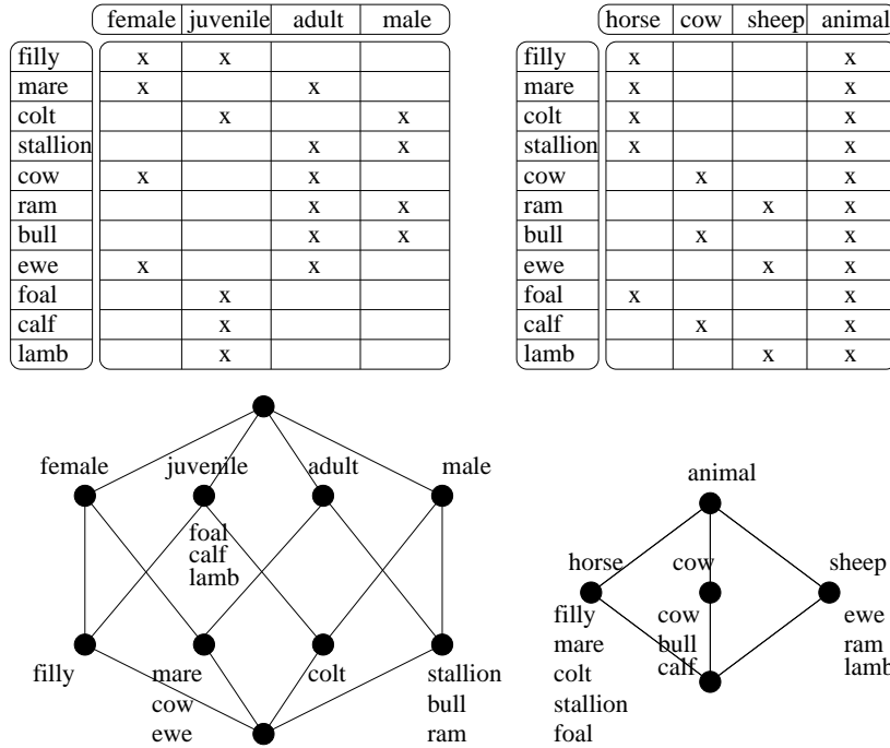
Figure 2: Formal contexts and line diagrams of their concept lattices
